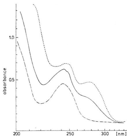
Fig. 5. Vapour phase ultraviolet absorption spectra, at temperatures indicated in brackets, of: —, 9-ethylhypoxanthine (270 °C); ---, 1,9-dimethylhypoxanthine (200 °C); - · - · -, 6-methoxy-9-methylpurine (320 °C).
